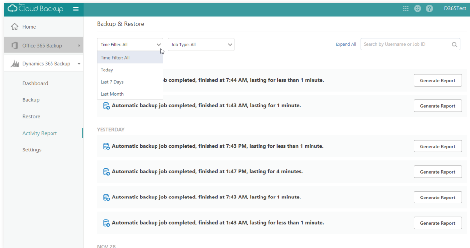
Job Monitoring
