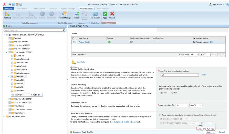
Apply Rules
