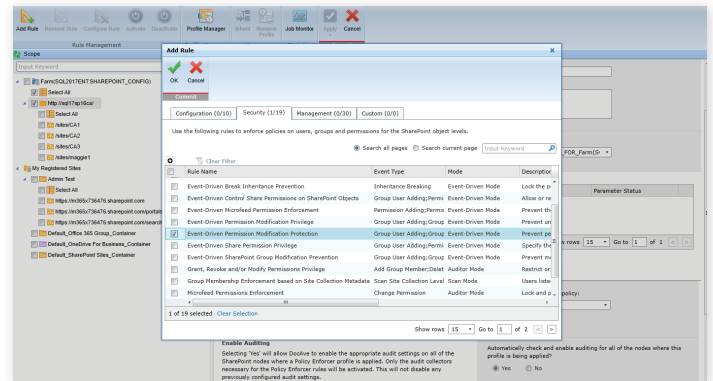
Add Rules
