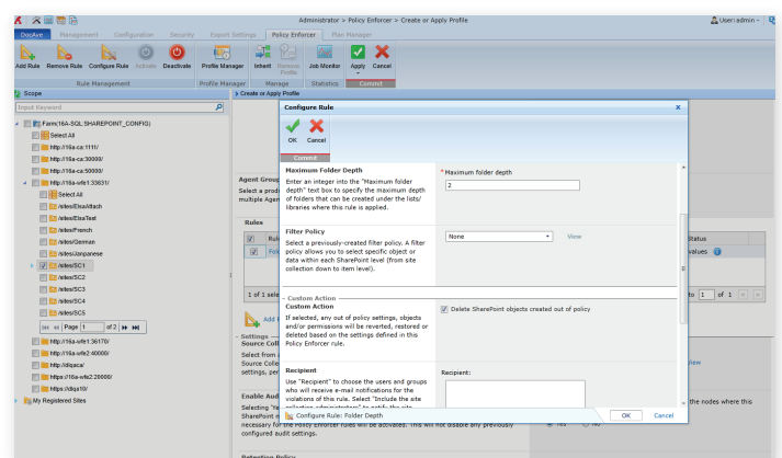
Configure Rules
